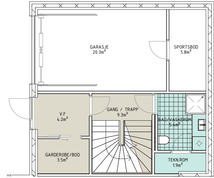
PLAN U
