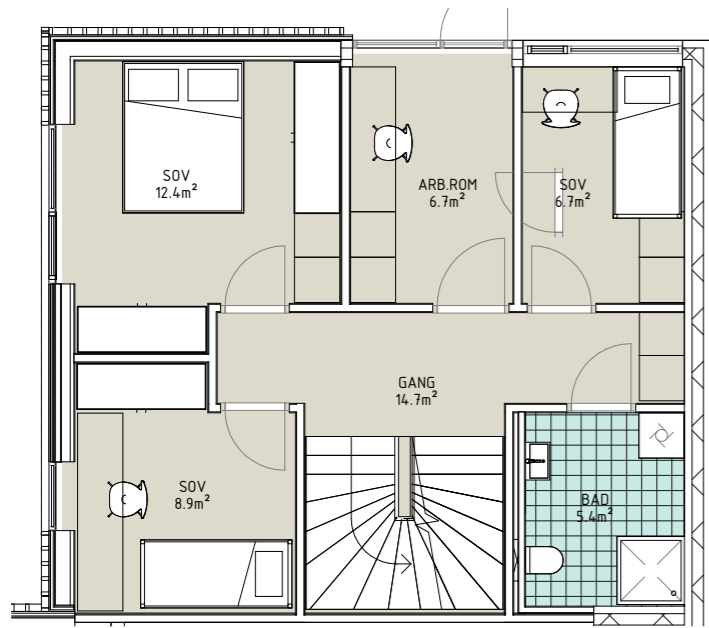
PLAN 1
